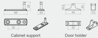
Cabinet support
