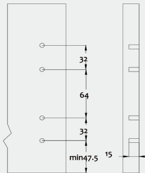
Front panel drilling dimensions
