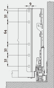
Back panel installation dimensions
