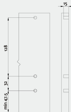
Front panel drilling dimensions
