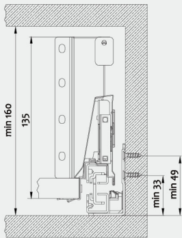
Cabinet space requirements
