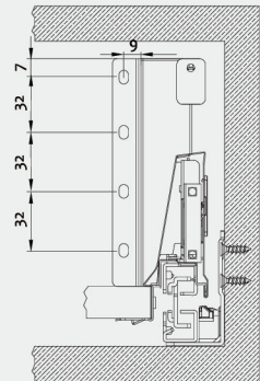
Back panel installation dimensions
