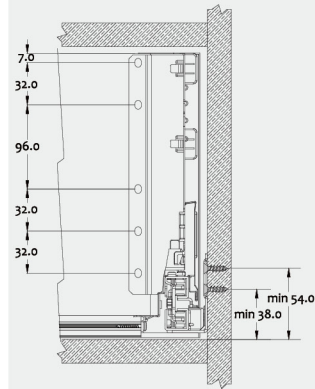
Back panel installation dimensions
