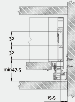
Front connector panel installation dimensions
