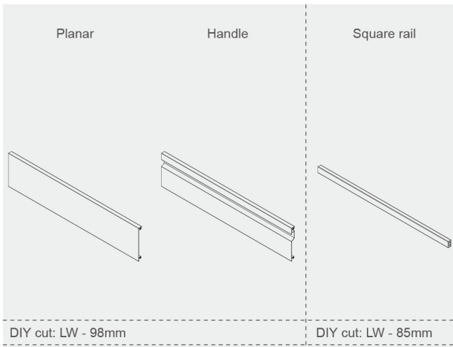
Back panel installation dimensions
