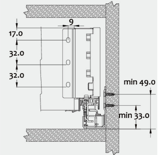
Back panel installation dimensions
