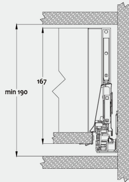
Cabinet space requirements
