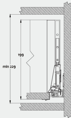
Cabinet space requirements
