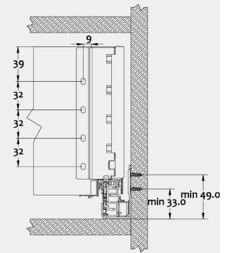
Back panel installation dimensions
