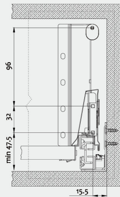
Front connector panel installation dimensions
