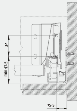
Front connector panel installation dimensions
