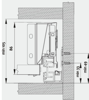
Cabinet space requirements
