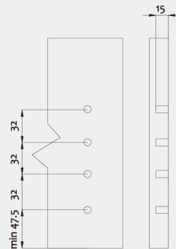
Front panel drilling dimensions
