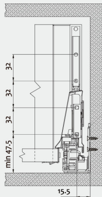
Front connector panel installation dimensions
