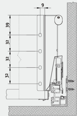
Back panel installation dimensions
