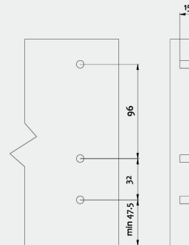
Front panel drilling dimensions
