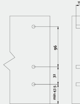
Front panel drilling dimensions
